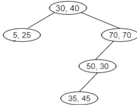
Fig. 3.4 KD tree in SDBMS
