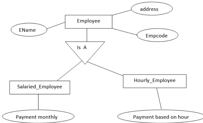
Fig.-15: Specialization
