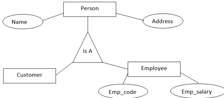
Fig.-14: Generalization
