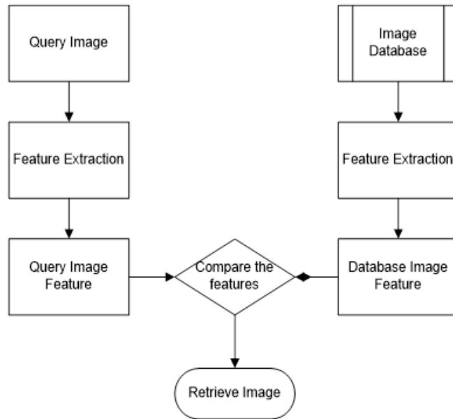
Fig. 3.2: CBIR system
